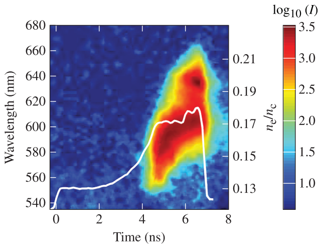
FIG. 12. Stimulated Raman scattering spectrum obtained on shot N140816 using the FABS in quad Q31B at a polar angle of \theta = 152^\circ . The white line is the incident laser power in the experiment.
