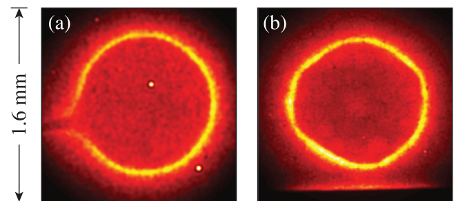
FIG. 8. Self-emission images of an imploding PDD capsule on shot N131210 as seen from (a) the polar direction at 7.0 ns and (b) the equator at 7.3 ns.
