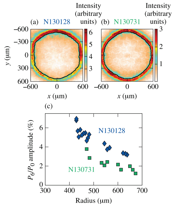
FIG. 9. Demonstration that improved symmetry can be obtained by tuning beam pointing and the power balance between NIF cones. [(a),(b)] Equatorial self-emission images of shots N130128 (before retuning) and N130731 (after retuning), both at a convergence ratio of \sim 2 . (c) P_6 amplitude normalized to the shell radius as a function of the shell radius, with time going from right to left. Shot N130128 [(a) and diamonds in (c)] exhibits a pronounced P_6 amplitude, which was reduced by \sim 50\% in N130731 [(b) and squares in (c)].
