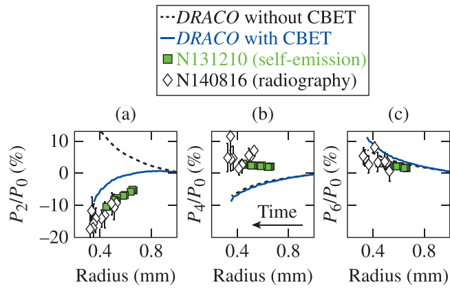
FIG. 7. Equatorial shape evolution of an imploding PDD capsule. Modal amplitudes normalized to the shell radius are shown for (a) P_2 , (b) P_4 , and (c) P_6 . Data are plotted as a function of shell radius, with time going from right to left. Diamonds are extracted from radiography data of shot N140816; squares are extracted from self-emission images on shot N131210. Lines show 2-D DRACO simulation results for shot N131210 with (solid) and without (dashed) CBET in the calculations.
