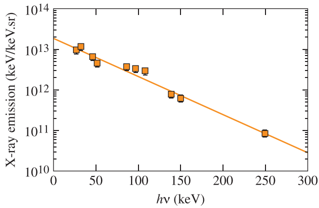
FIG. 11. Time-integrated FFLEX analysis for shot N131210. The squares denote total emission as measured by the FFLEX detector; the solid line is the fitted x-ray spectrum giving a hot-electron component in the experiment at a temperature of 46 \pm 2 keV and with a total energy content of 2.5 \pm 0.3 kJ.
