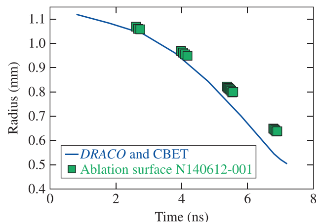
FIG. 10. Comparison of trajectory data extracted from self-emission images (squares) and 2-D DRACO simulations with CBET (solid line).
