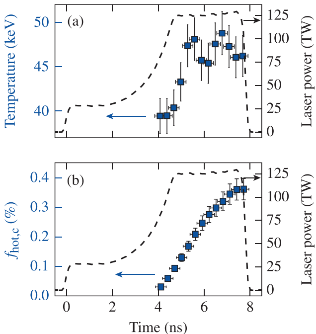
FIG. 13. Time-resolved FFLEX analysis for shot N131210 (compare Fig. 12). The dashed line is the total incident laser power. (a) The hot-electron temperature; (b) the time-resolved, total conversion efficiency of incident laser energy into hot electrons. At the end of the laser pulse, \sim 0.4\% of the incident energy has been converted into energetic electrons.
