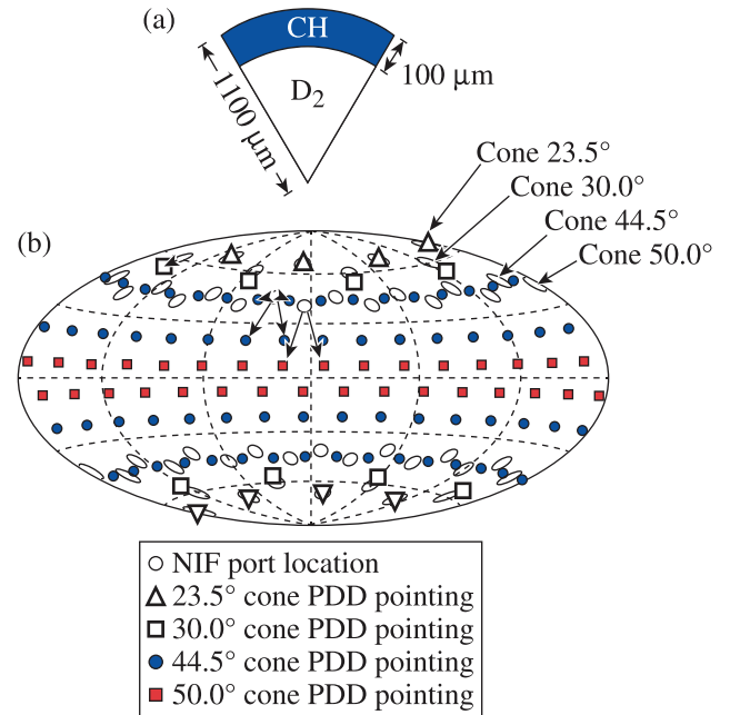
FIG. 3. (a) Typical target used for the first series of PDD experiments on the NIF. (b) Beam pointing in PDD experiments, illustrated with respect to the initial target surface. Open circles denote original port locations. See also Table I.
