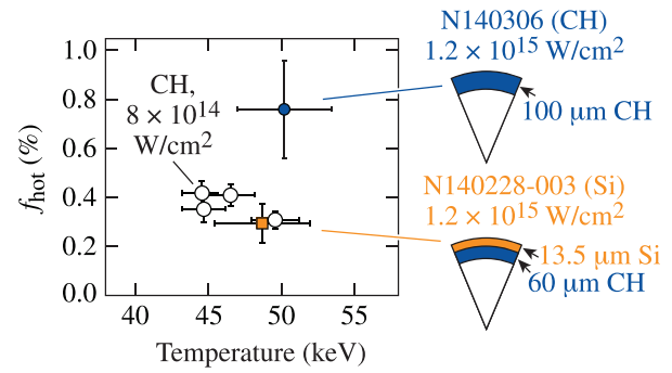
FIG. 14. Hot-electron fraction from six PDD targets, mostly CH, irradiated with nominal peak irradiance of 8 \times 10^{14} W/cm 2 (open circles). Two shots were taken at 1.2 \times 10^{15} W/cm 2 ; one with a CH ablator (solid circle), one with a Si ablator (solid square).
