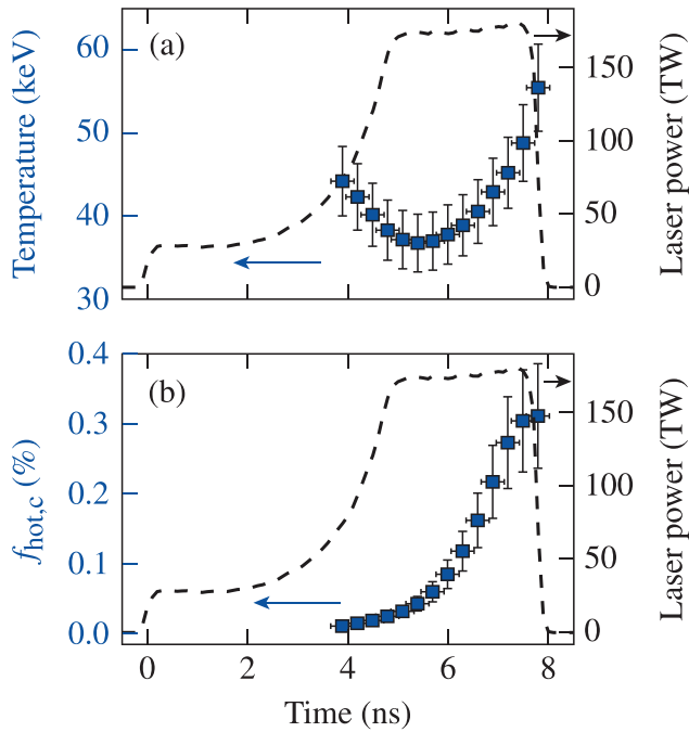
FIG. 15. Time-resolved FFLEX analysis for the Si-ablator experiment at a peak irradiance of 8 \times 10^{14} \text{ W/cm}^2 (shot N140228-003). The dashed line is the total incident laser power. (a) The hot-electron temperature; (b) the time-resolved, total conversion efficiency of incident laser energy into hot electrons. At the end of the laser pulse, \sim 0.3\% of the incident energy has been converted into energetic electrons.
