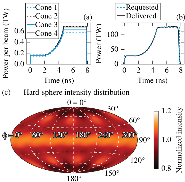
FIG. 4. (a) Pulse shapes in each cone for shot N131210 comprising a low foot to set the shell adiabat followed by a slow rise to peak irradiance. (b) Comparison between requested and delivered total pulse shapes. (c) Hard-sphere projection of the irradiance distribution at the initial target radius. The irradiance is increased near the equator to compensate for the reduced hydroefficiency of the energy deposited there.
