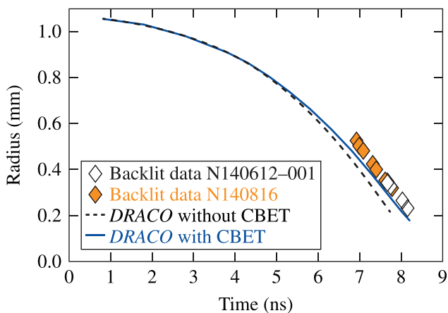
FIG. 6. Two-dimensional DRACO simulations that do not include CBET (dashed line) do not match the experimental shell trajectory extracted from radiography data (diamonds, shots N140612-001 and N140816). By including CBET, the agreement improves (solid blue line).
