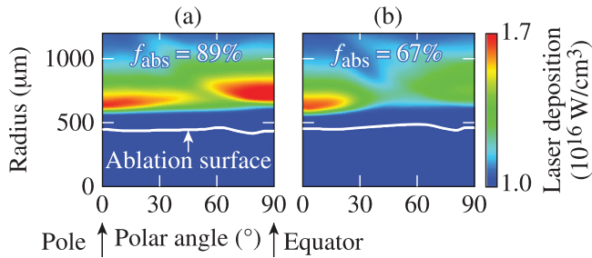
FIG. 2. Calculated instantaneous deposited laser power for polar-direct-drive shot N130128 at 6.5 ns using the 2-D code DRACO : (a) collisional absorption only and (b) including CBET. The integrated absorption in the presence of CBET is reduced by \sim 20\% . 30 Reproduced with permission from Radha et al. , J. Phys. Conf. Ser. ■ Copyright ■ IOP Science.
